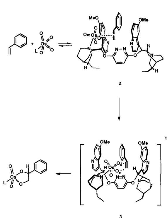
Scheme 1. CCN [3+2] cycloaddition pathway for the asymmetric dihydroxylation of styrene catalyzed by 1\bullet\text{OsO}_4 .
