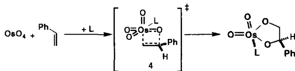
Scheme 2. The [2+2] cycloaddition pathway for the asymmetric dihydroxylation of styrene.
